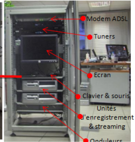
A Rack model for media Transfer in a region containing one Radio service
